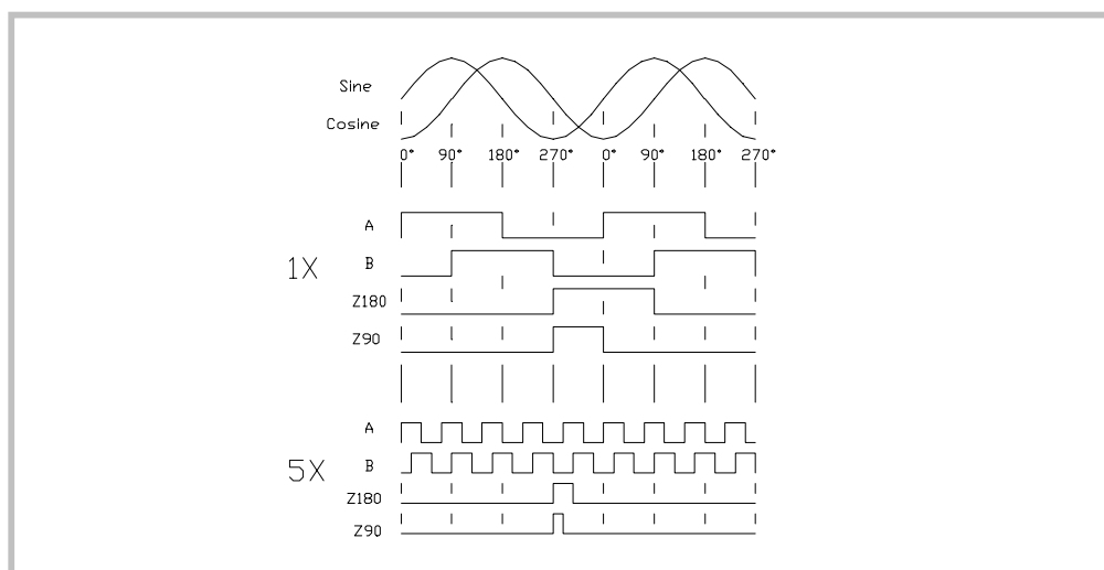
Timing Diagram
